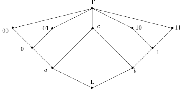
FIGURE 1. A finite lattice P such that \mathcal{C}(P) is not a lattice
